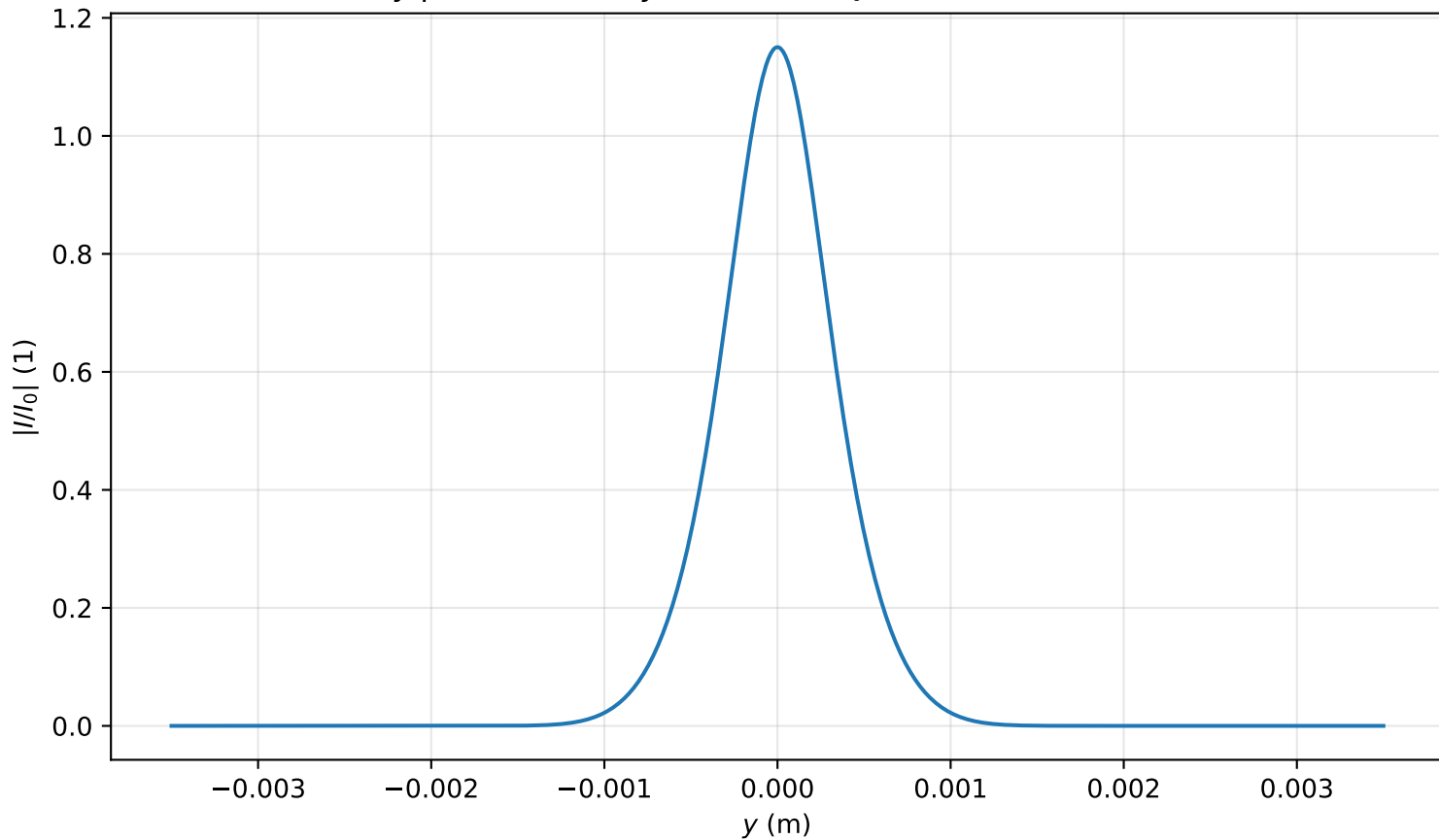
Intensity profile I(x=0, y, z=0.716)/I_0 , P_{in}=0.7P_{cr} , artificial time
